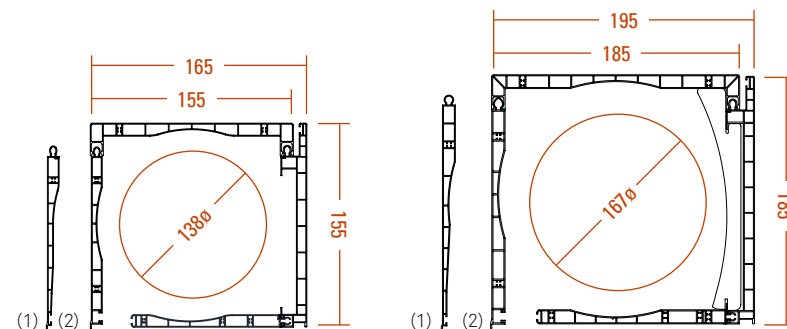
CAJÓN PVC ENERGY CUBE 155
