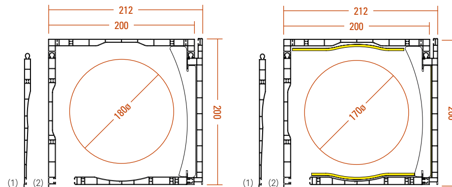
CAJÓN PVC ENERGY CUBE 200
